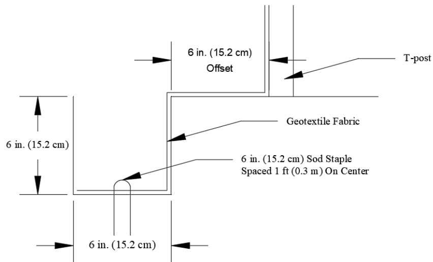
Offset Trench Detail
