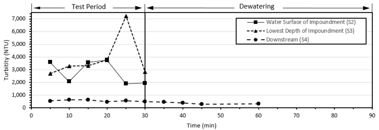
(a) average turbidity over time for the first simulated runoff event for each installation
