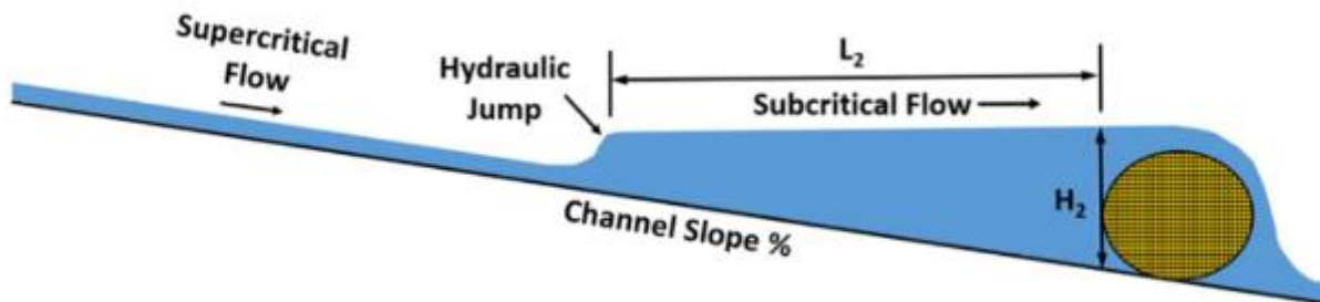
(b) Measured impoundment depth and length
