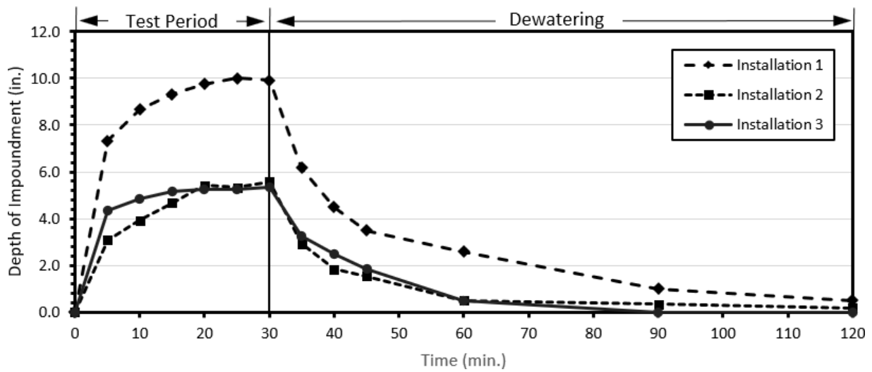
(a) Depth of Impoundment
