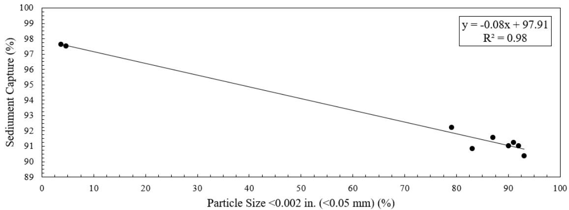
Figure 2.6: Average Sediment Capture by Percent Fines
