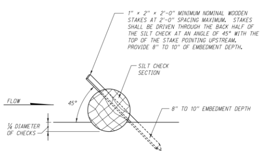
(a) option A for installation
