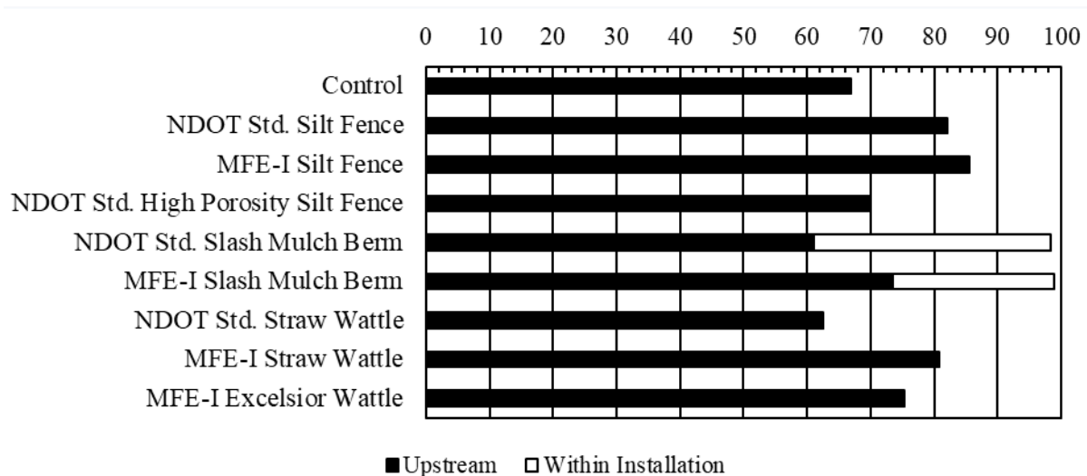
Figure 3.36 Average Sediment Capture for Standard and Modified Sediment Barrier Installations
