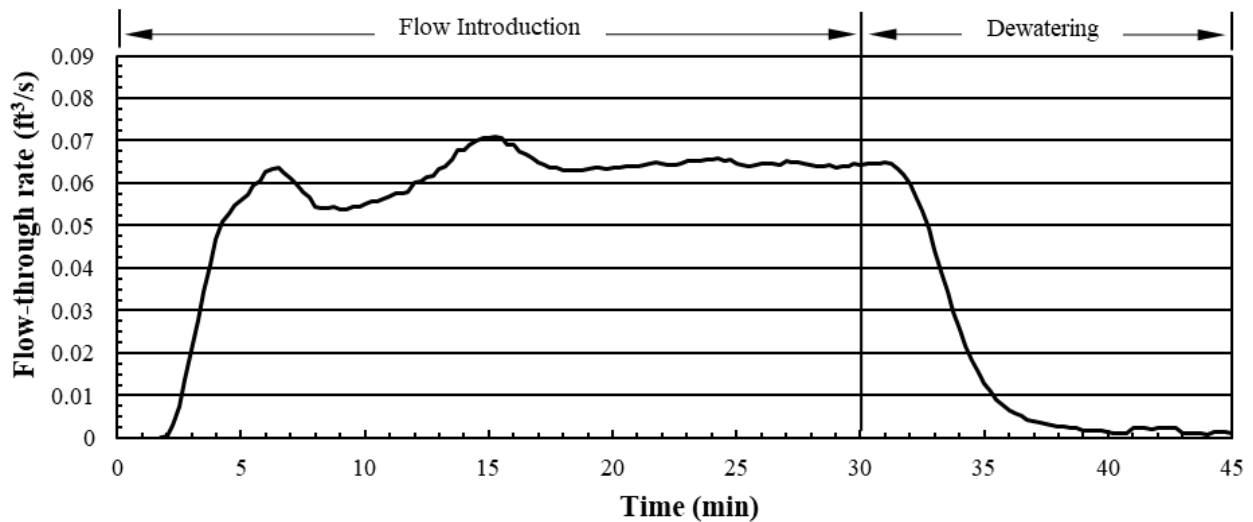
Figure 3.32 Flow through Excelsior Wattle Installations
