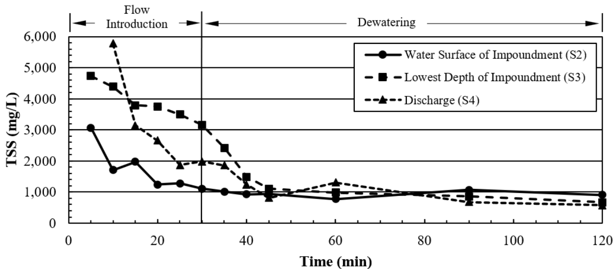
(b) Average TSS over time for woven silt fence installations
