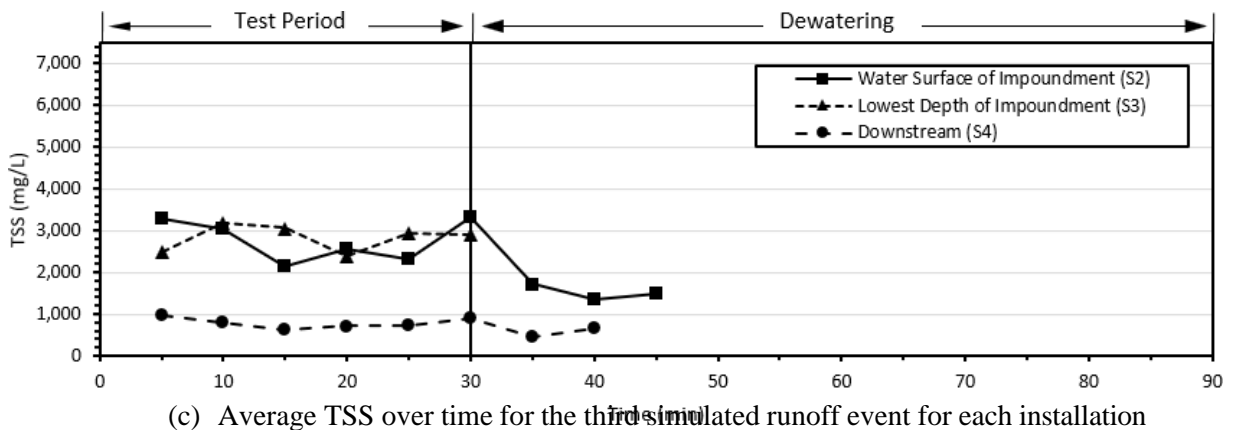
Figure 9: TSS over Time.
