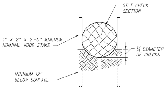
(c) option C for installation
