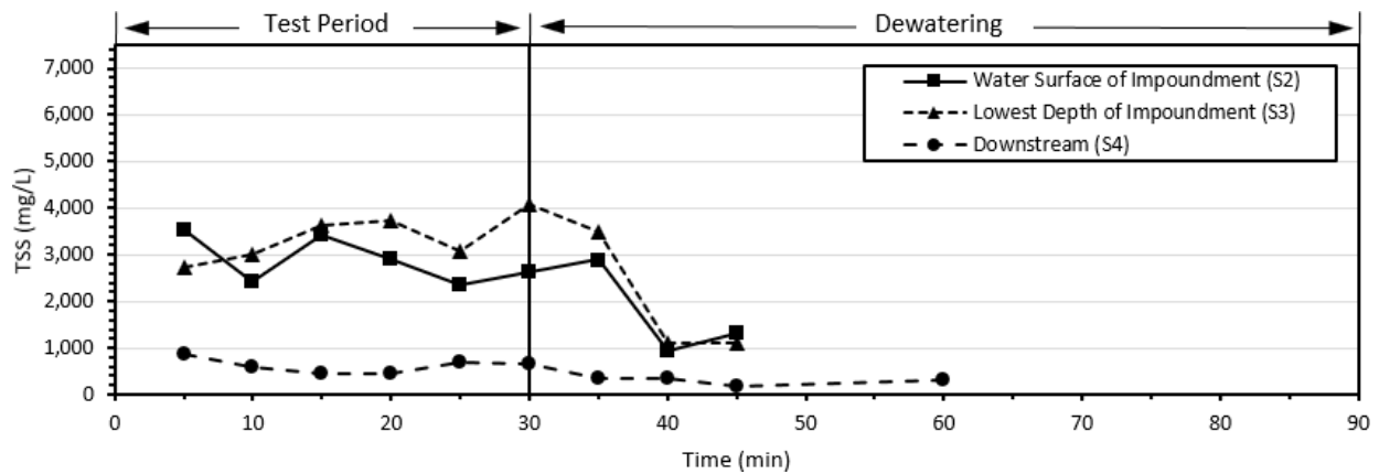
Figure 10: Average TSS over Three Tests.
