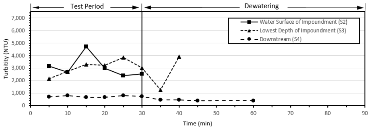
Figure 8: Average Turbidity across all Three Installations.
