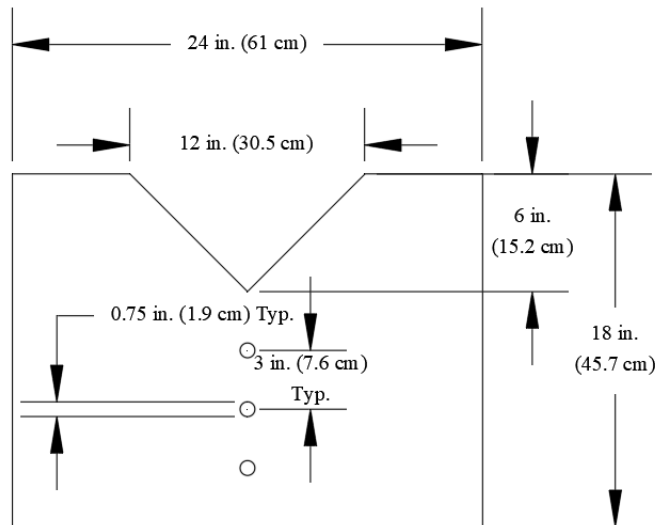
Dewatering Board w/ Overflow Weir Detail
