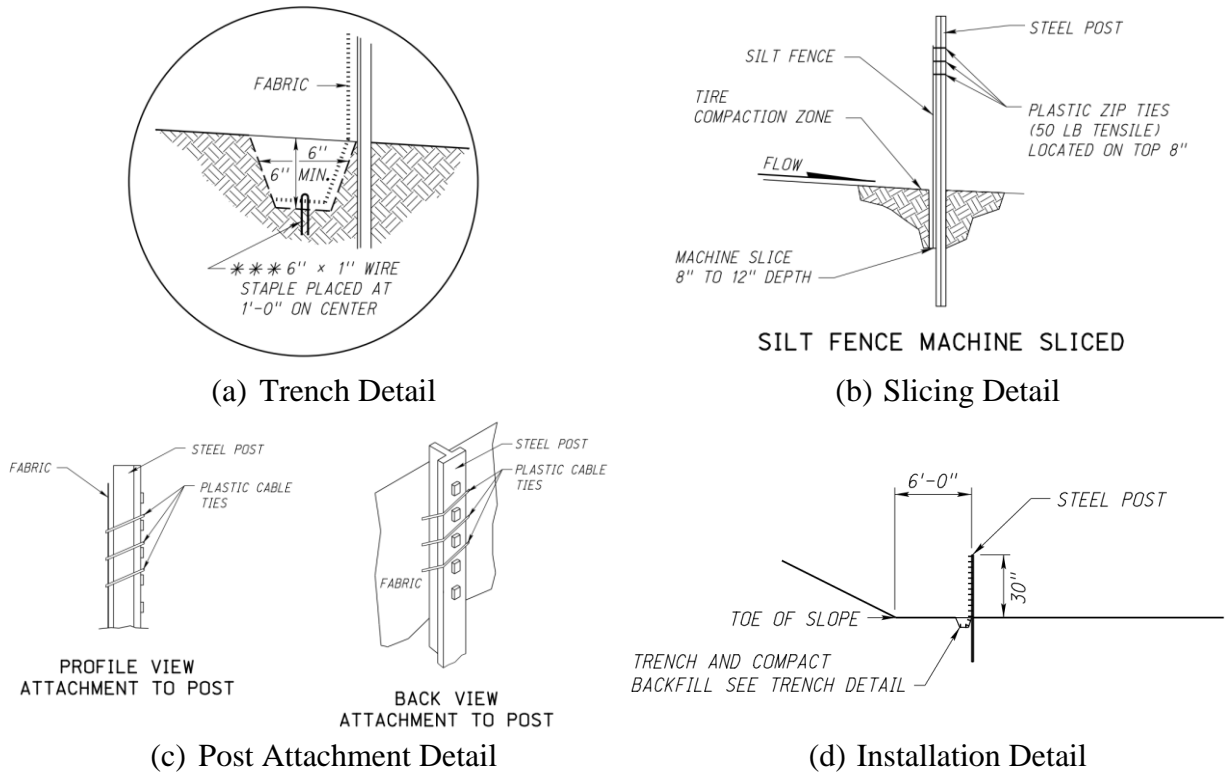
Figure 3.2 Nebraska DOT Silt Fence Installation Details
