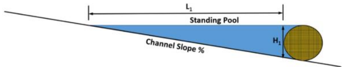
(a) Theoretical impoundment depth and length
