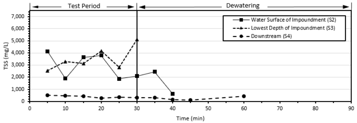
(a) Average TSS over time for the first simulated runoff event for each installation
