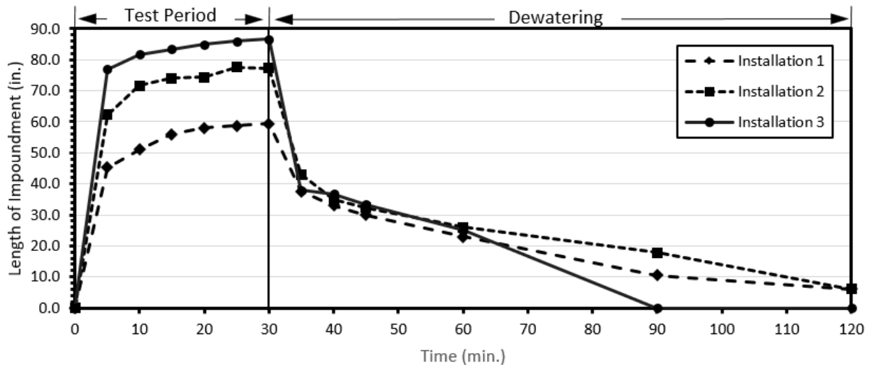
Figure 6: Impoundment Depth and Length.
