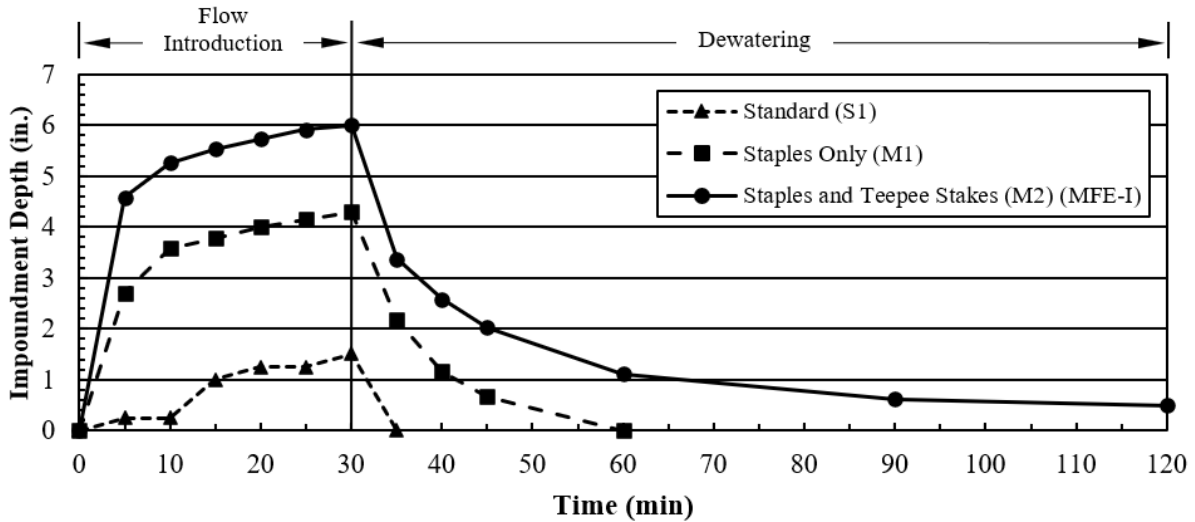
Figure 3.29: Average Impoundment Depth for Straw Wattle Installations
