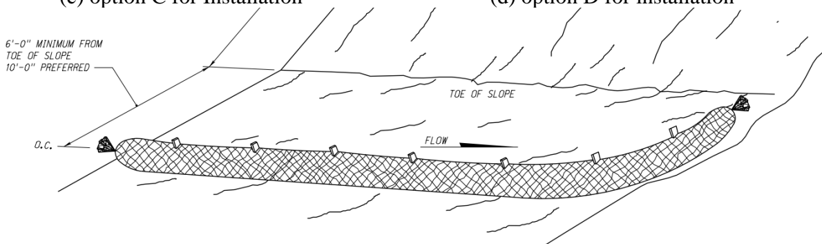
(e) installation detail at toe of slope
