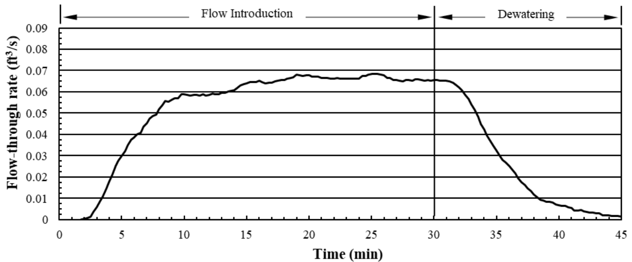
Figure 3.30 Average flow rate through Straw Wattle MFE-I Installations
